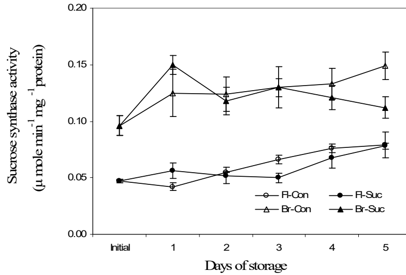
Figure 2. Changes in sucrose synthase activity in broccoli head supplied with exogenous sucrose during storage at room temperature. Legend: as shown in Fig. 1.
