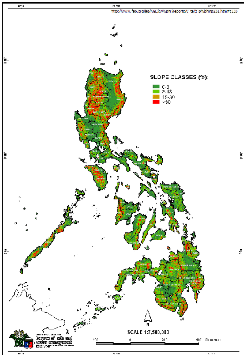
Fig.1. Slope classes in the Philippines
