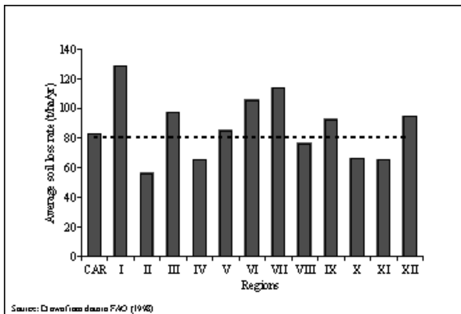
Fig. 2. Average erosion rate by region in the Philippines in 1993. Dotted line represents the average erosion rate
